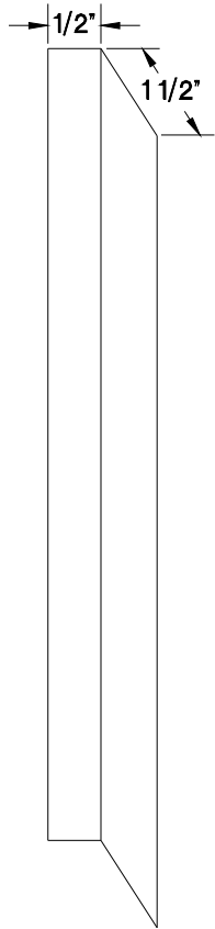
INTERIOR WINDOW TRIM. USE TO SECURE 2" THICK DISPLAY WINDOWS IN 4" THICK INSULATED WALL PANELS
