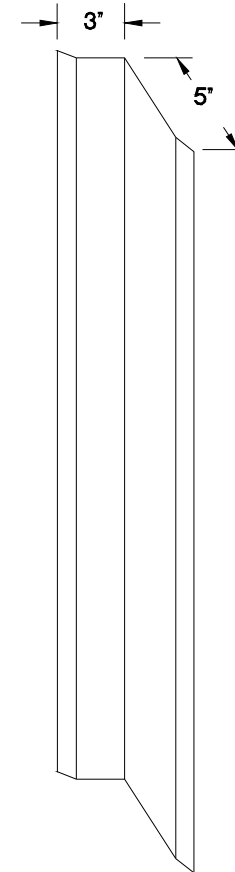
CORNER TRIM STRIP. USE TO ENCLOSE GAP BETWEEN WALL OF COOLER AND BUILDING WALL
