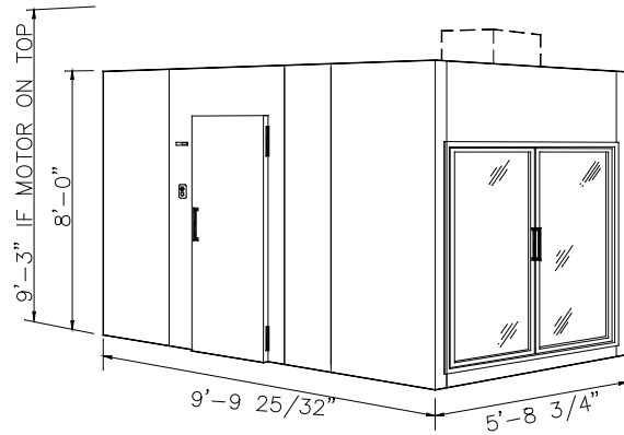
PERSPECTIVE
