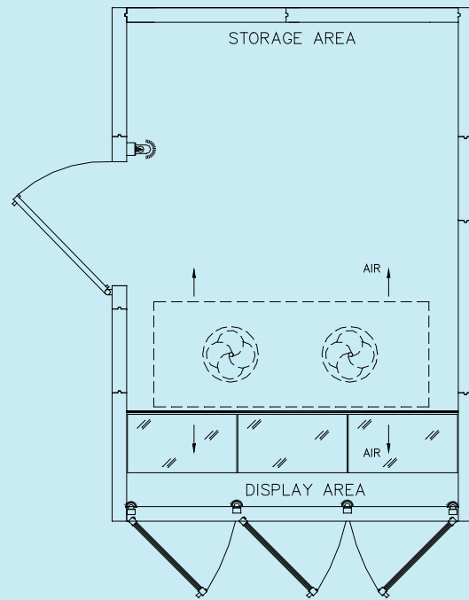
PLAN VIEW
